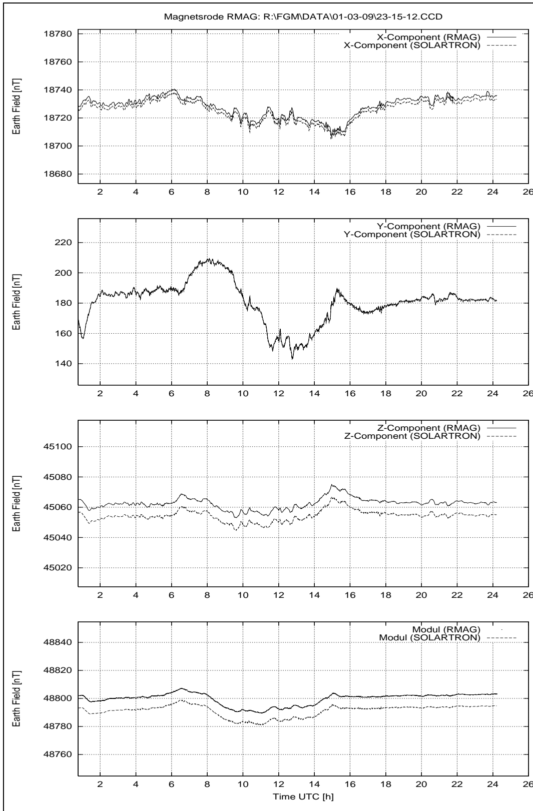
Figure 184: March 9, 2001: Earthfield variations.
