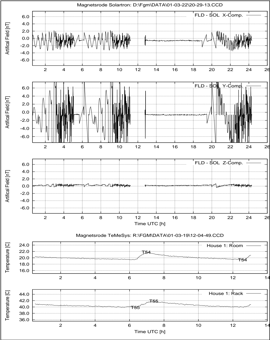
Figure 14: March 22, 2001: System Performance: FLD – SOL; Temperatures at House 1.
