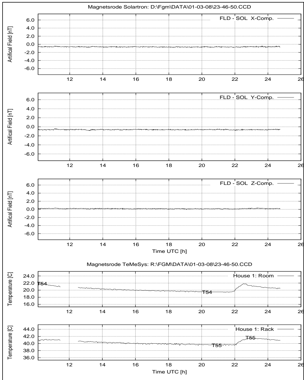
Figure 177: March 8, 2001: System Performance: FLD – SOL; Temperatures at House 1.
