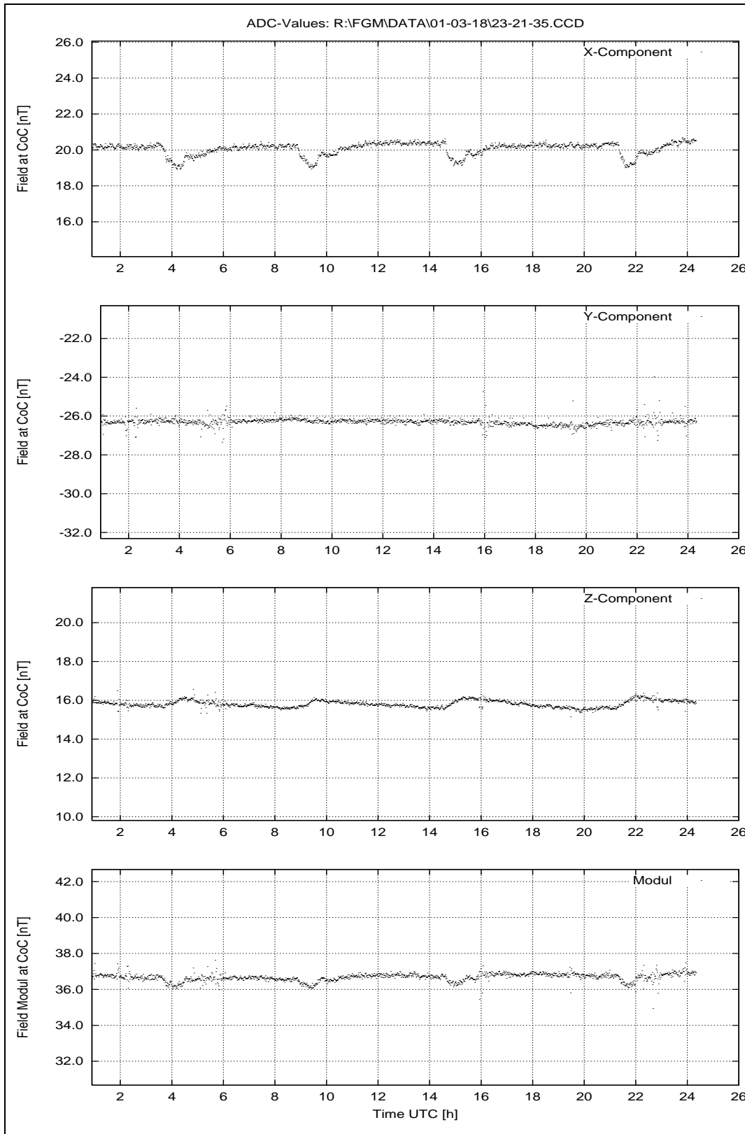
Figure 218: March 18, 2001: Zero field at CoC.
