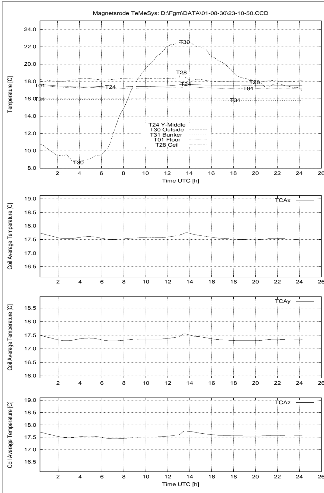
Figure 125: August 30, 2001: Temperatures House 2.
