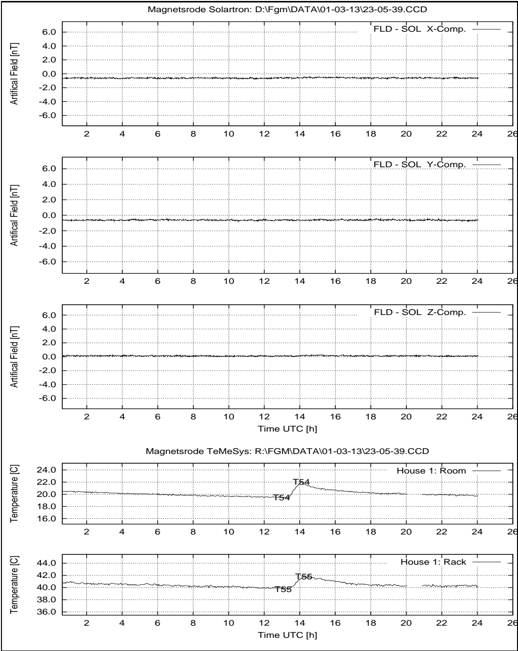
Figure 197: March 13, 2001: System Performance: FLD – SOL; Temperatures at House 1.
