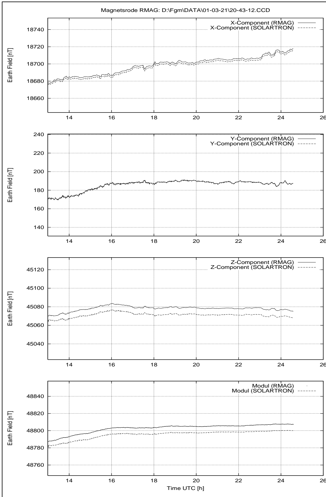
Figure 13: March 21, 2001: Earthfield variations.
