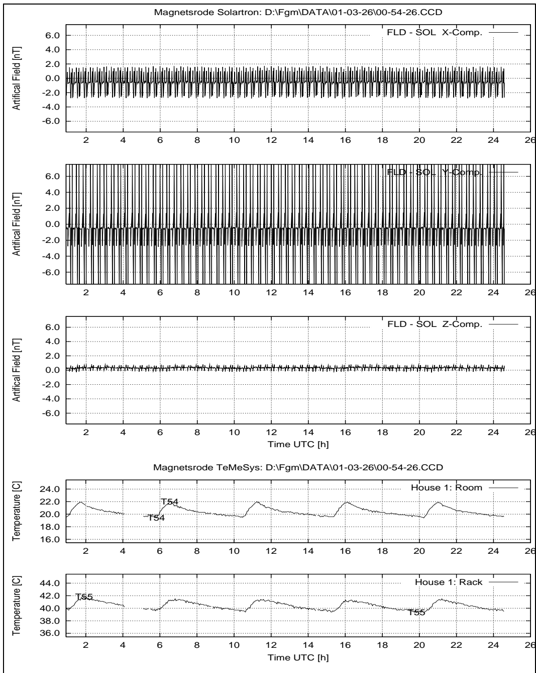
Figure 30: March 26, 2001: System Performance: FLD – SOL; Temperatures at House 1.
