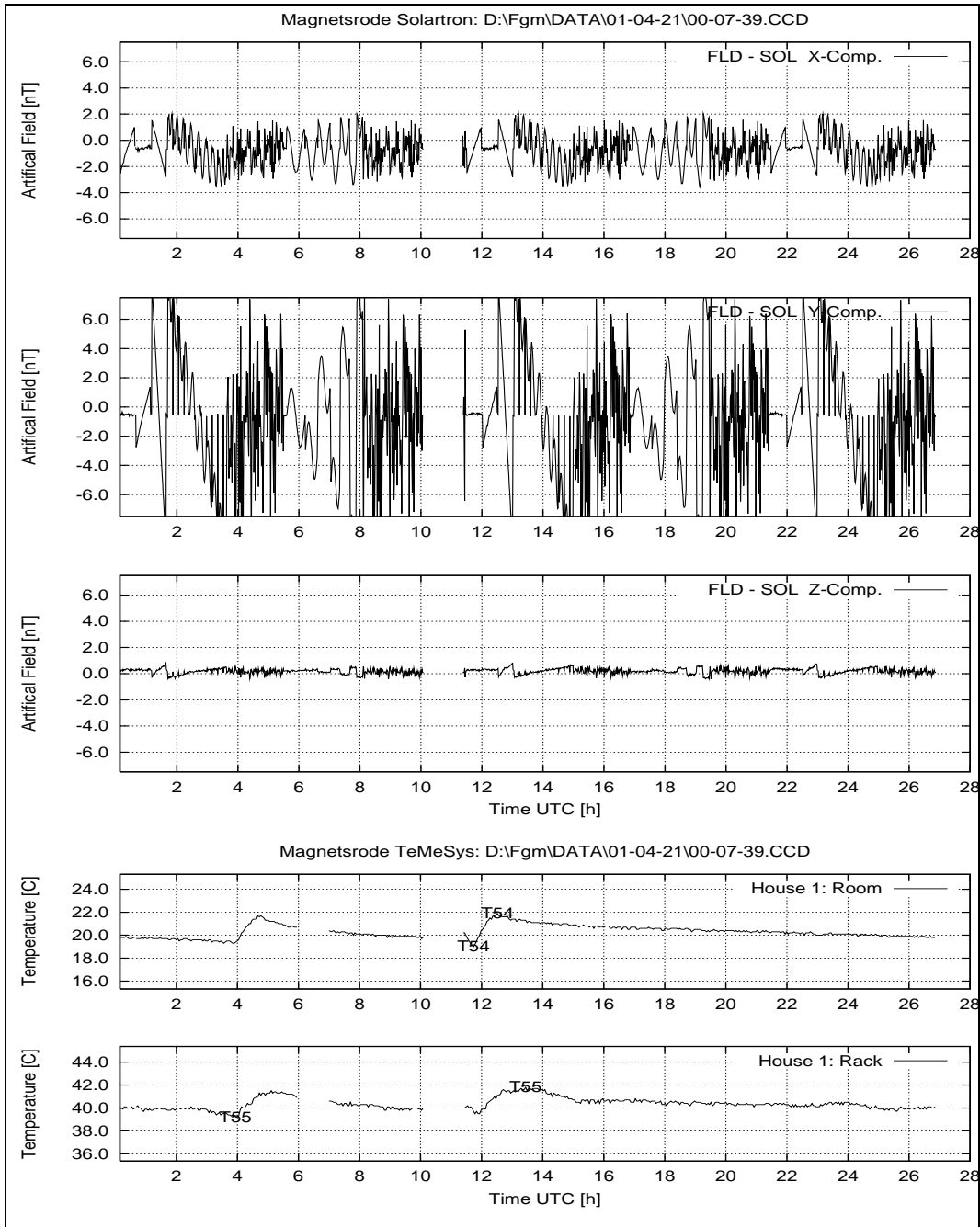
Figure 61: April 21, 2001: System Performance: FLD – SOL; Temperatures at House 1.
