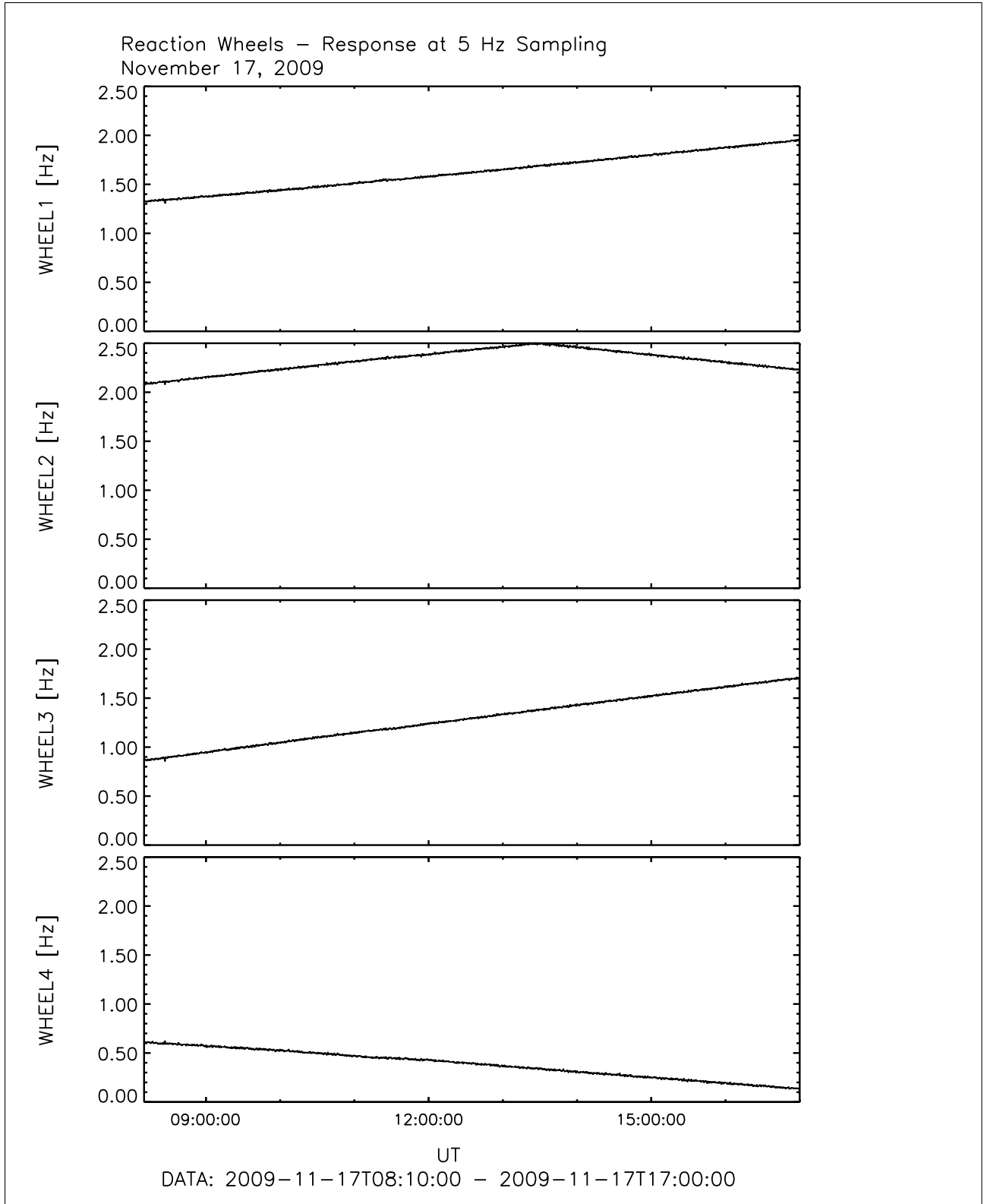
Figure 11: File: wheels_5Hz_Sampling2009-11-17T08-10
