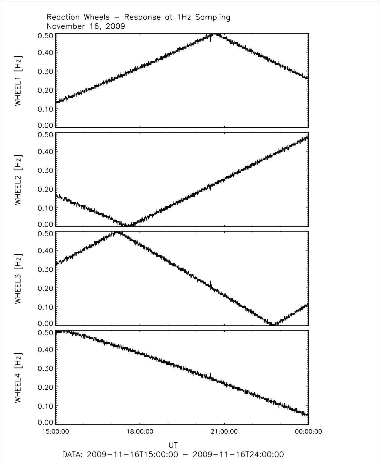
Figure 7: File: wheels_1Hz_Sampling2009-11-16T15-00
