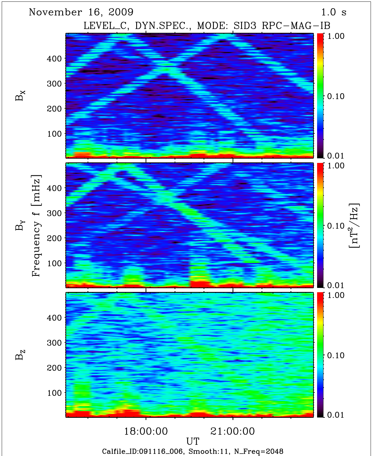
Figure 2: File: RPCMAG091116T1501_CLC_IB_M3_DS0_10000_006
