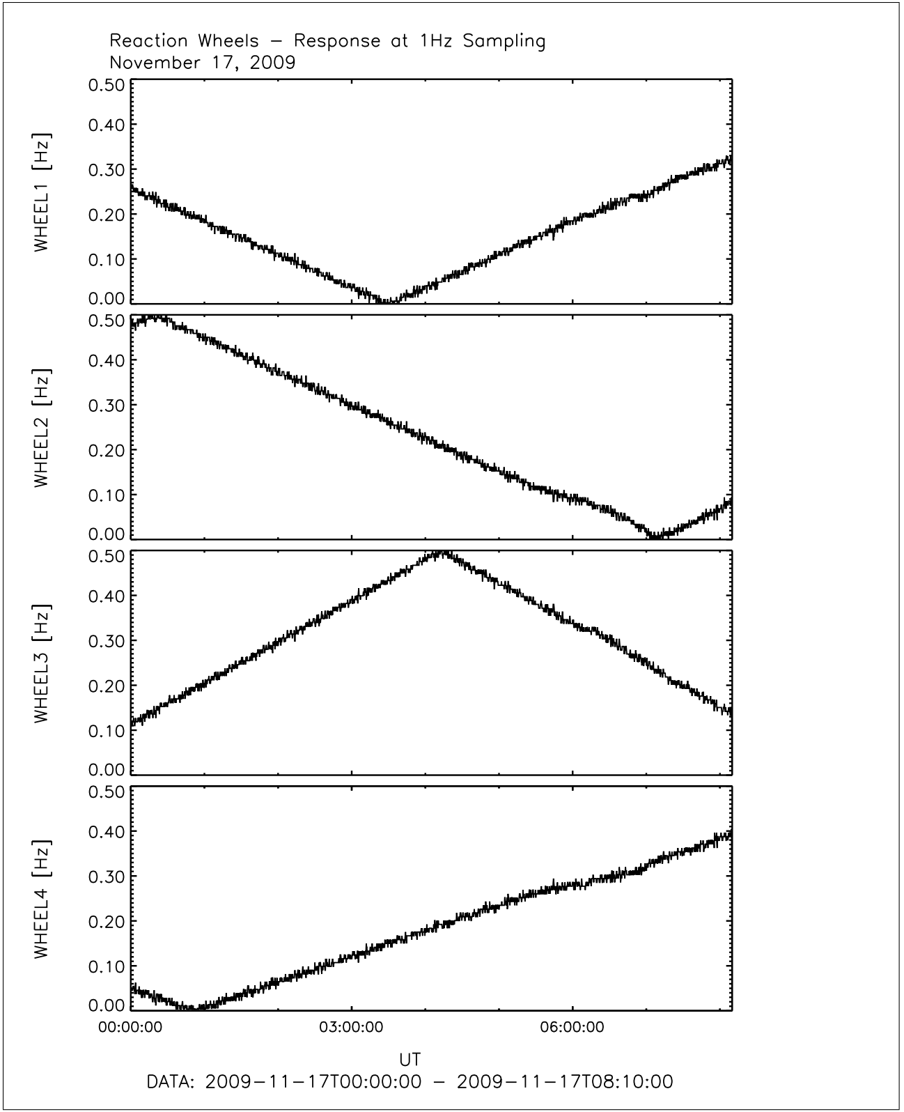
Figure 9: File: wheels_1Hz_Sampling2009-11-17T00-00
