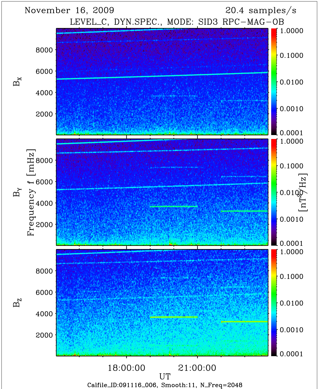
Figure 1: File: RPCMAG091116T1501_CLC_OB_M3_DS0_10000_006
