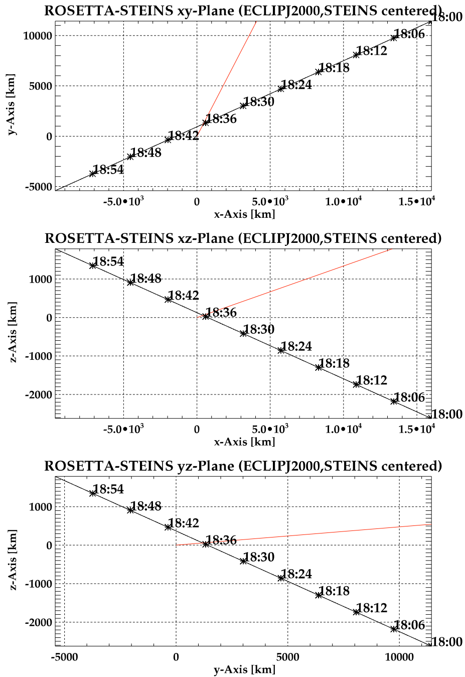
Figure 2: ROSETTA'S Fly-By Trajectory in ECLIPJ2000 coordinates. Red Line: SUN Direction
