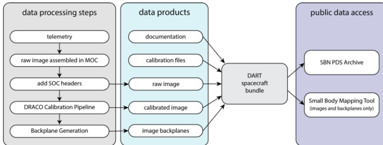
Figure 9. DRACO data processing flow diagram.
