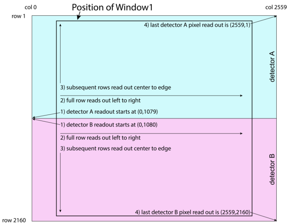
Figure 5. Diagram of the DRACO detector, indicating pixel numbering, readout direction, and the position of Window1 (see Section 4.1.4.1). Rows are numbered starting from 1 to account for the header row (see Section 4.1.4). Corresponding pixels from both halves are read out simultaneously. Note, to show an image as an observer looking out the DRACO boresight would see, it has to be flipped vertically to place the origin at the lower left (see Section 4.1.6.2).
