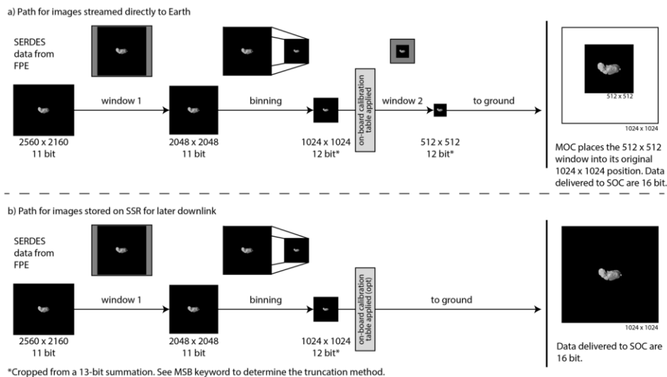
Figure 7. The path of an image through the DRACO on-board image processing pipeline for images sent to a) the radio for downlink to Earth (e.g., Terminal and Final phase images) and b) the SSR for downlink at a later time (e.g., OpNav, calibration, lightcurve images). See Table 4 for a full record of which types of images took which path.
