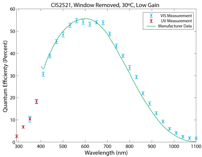
Figure 4. Quantum efficiency of the DRACO detector.
