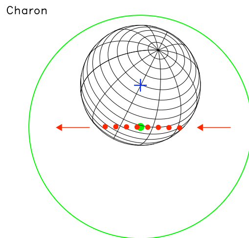
Figure 8. View of Charon nightside from the NH spacecraft during Earth occultation. See similar sketch of the Pluto occultation geometry for explanations of the various features. A major difference at Charon with respect to the Pluto occultation is that the 3-dB beam is now much larger than the Charon disk.
