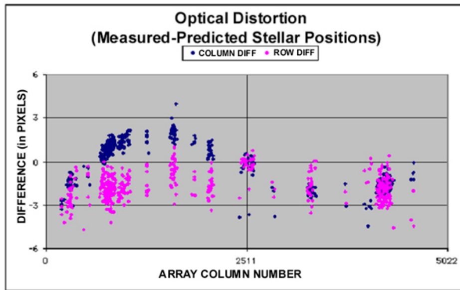
Figure 12: Effect of optical distortion for MVIC framing camera. The plotted points are the differences between predicted row and column stellar positions and true row and column stellar positions as determined using dense star fields. The differences are plotted as a function of array column number.
