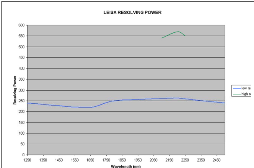
Figure 8: Measured resolving power ( \lambda/\Delta\lambda ) of the LEISA array/filter assembly for the lower-resolution (1.25 – 2.5 \mu\text{m} ) and higher-resolution (2.1 – 2.25 \mu\text{m} ) segments.
