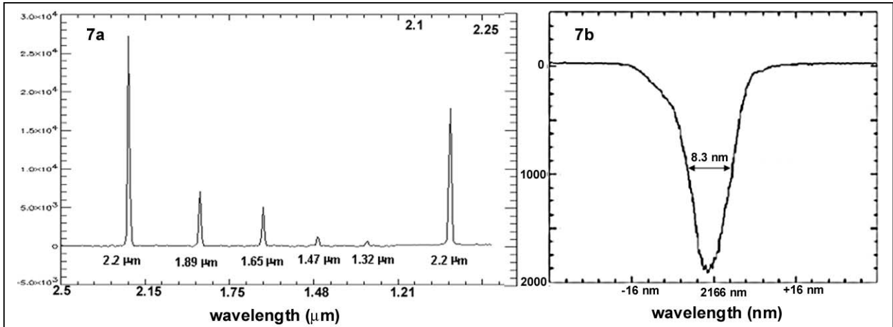
Figure 7: (a) A single row of LEISA showing multiple orders of a grating. Note the non-linear (logarithmic) wavelength scale and the presence of the 2.2 \mu\text{m} order in both the low resolution (2.5 to 1.25 \mu\text{m} , \lambda/\Delta\lambda \sim 240 ) and the high resolution (2.1 to 2.25 \mu\text{m} , \lambda/\Delta\lambda \sim 560 ) filter segments. (b) Wavelength dependence of transmitted intensity (instrument lineshape function) at a single pixel as the wavelength is varied from 2133 to 2200 nm in 0.3 nm steps.
