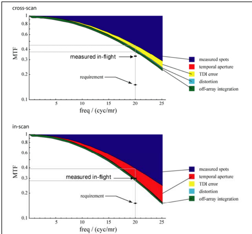
Figure 11: Modeled and measured MTF for the MVIC panchromatic TDI channel. “Measured spots” represents the measured contribution of the optical characteristics to the MTF, while the other factors are based on predicted behavior at the 3\sigma level. The temporal aperture and the TDI error have to do with uncompensated spacecraft motion. Off array integration is a term that comes about because of insufficient masking of the bulk silicon from the light. The points labeled “measured in-flight” are derived from stellar observations and represent the full system MTF. These clearly exceed the requirement.
