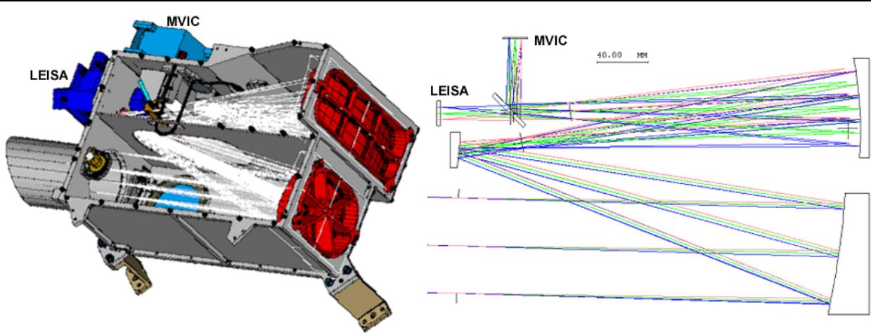
Figure 3: (Left) Interior of the Ralph TDA Showing the light path. Note the stainless steel tube loop forming the SIA fiber path. (Right) Raytrace diagram showing the path to the LEISA and MVIC focal planes.
