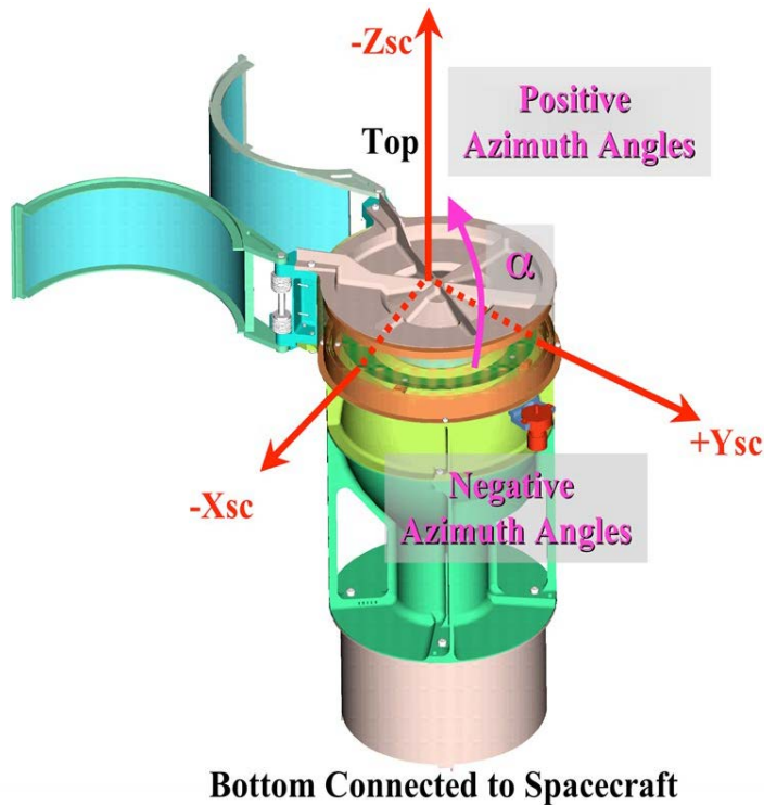
Figure 10: Diagram defining the azimuth angle. Bottom of the instrument connects to the spacecraft.
