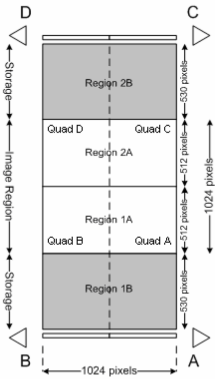
Figure 3 – CCD Architecture
