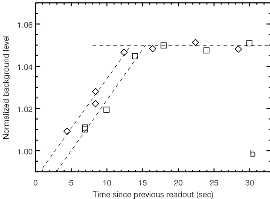
Figure 74 - Normalized background level as a function of the inter-sequence gap for the first image in a sequence in mode 1. a) The full range of observations, showing a constant overshoot level (dashed line) for longer gaps. b) Blowup of the first 33 seconds, showing the linear rise with time. The diamonds are measurements obtained for mode change from 2 to 1, and the squares are for no mode change (1-1). Linear fits to the rising portion in each of the two cases, indicated by the dashed lines, have the same slope but are offset in time. Refer to the text for more discussion.
