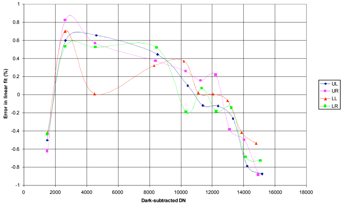
Figure 22 - Residuals to a linear fit of the HRI-VIS response
