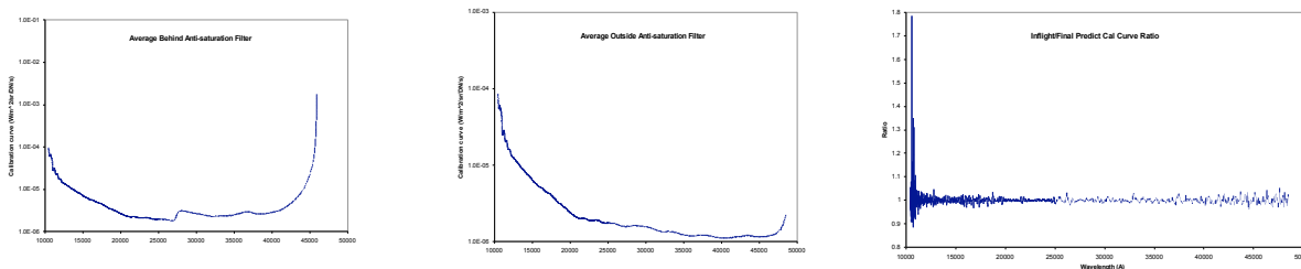
Figure 84 - Best-fit IR spectrometer calibration curves and their ratio to the inflight measurements
