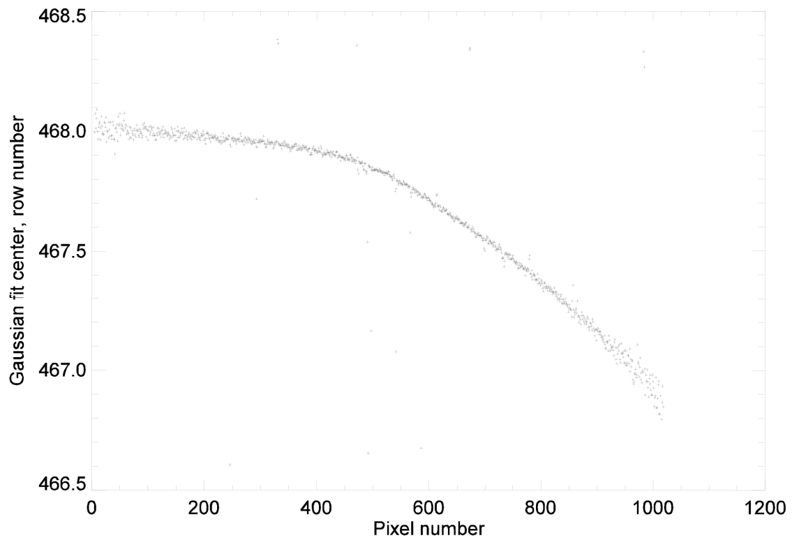
Figure 61 - The inflight variation of the centers of Gaussian fits of the calibration star Beta Hyi as a function of pixel number. The total variation from one edge of the IR detector to the other is almost exactly one physical pixel.
