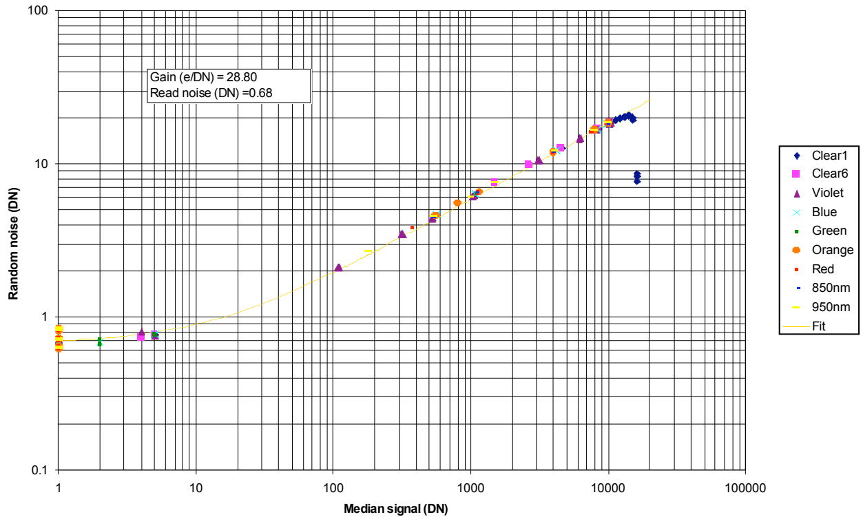
Figure 23 – Photon transfer data for HRI-VIS
