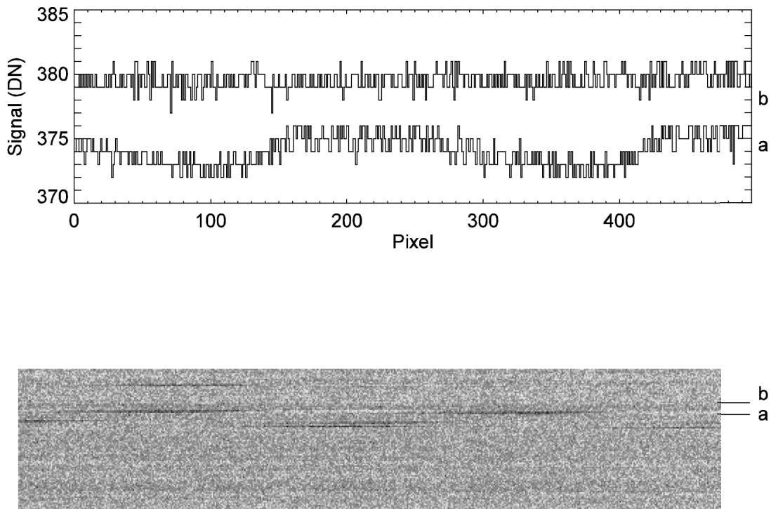
Figure 38 - An example of a recurring low-level noise seen in all three CCD imagers. A segment from one quadrant of an HRI CCD image is shown below, and two DN profiles across the image are plotted above. The duration of the noise corresponds to about two times the readout time for one row. Profile a) is a row with the noise, and profile b) is a row without the noise. Profile b) is offset by +5 DN for clarity.
