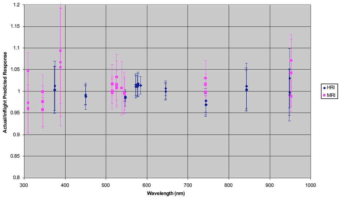
Figure 30 - Ratios of actual inflight stellar response rates to those predicted using the adjusted camera models
