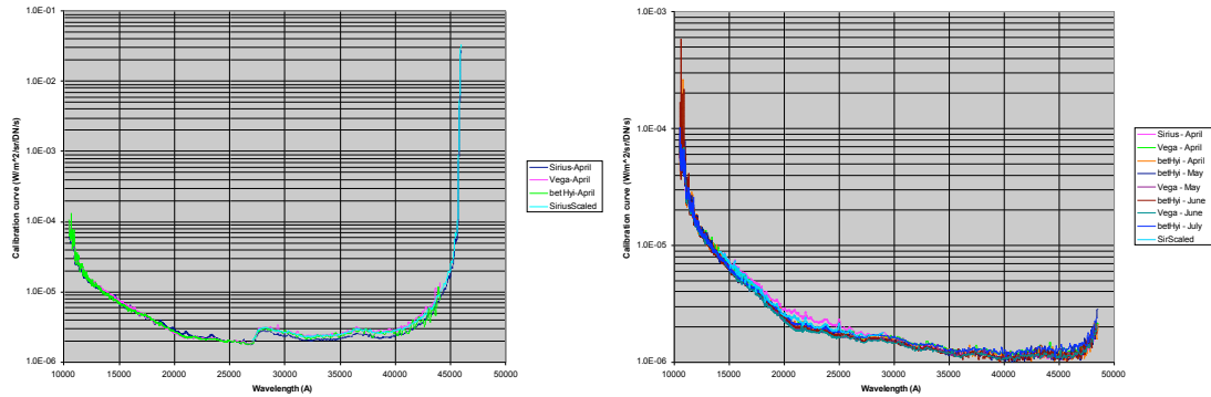
Figure 80 - IR inflight calibration curves; binned behind anti-saturation filter on left, unbinned outside anti-saturation filter on right
