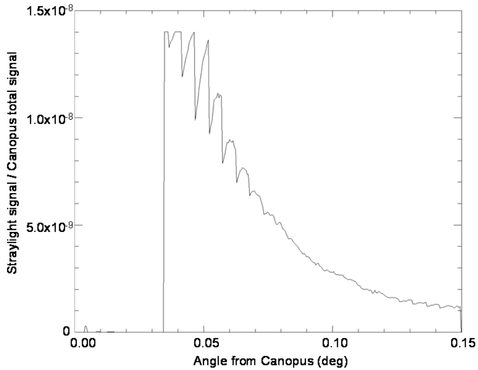
Figure 44 - One of the bright columns from the HRI polar plot in Figure 43 (at 94^\circ ) normalized with respect to the total Canopus signal showing the worst-case HRI scattered light response to a point source outside the FOV
