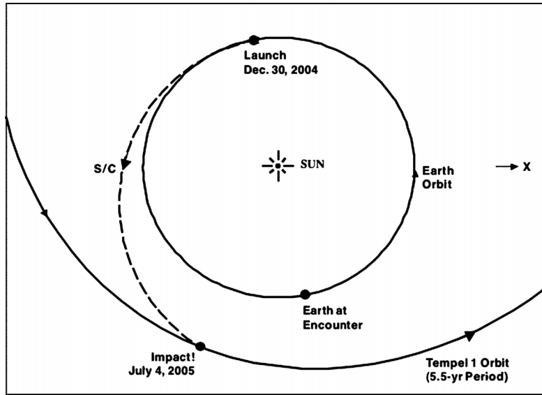
Figure 4. The Deep Impact interplanetary trajectory projected into the Ecliptic. A launch opportunity of 30 days begins on 30 December 2004, with a fixed arrival date at the comet of 4 July 2005.
